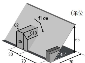
Fig.1 魚道模型 (突起なし) Fishway model (No protrusions)
